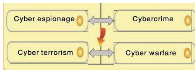
FIGURE 2. Cyber Attack
